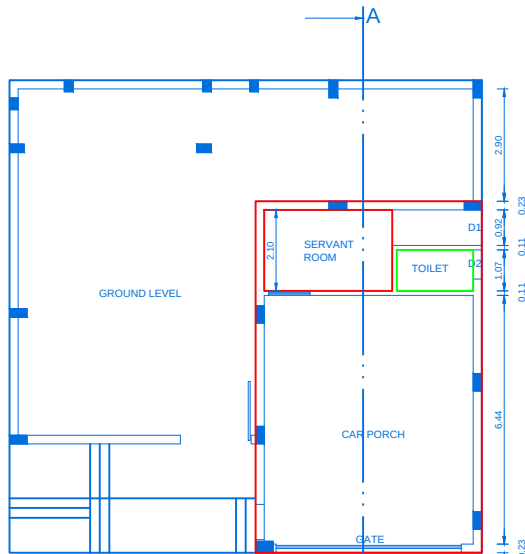
STILT FLOOR PLAN
