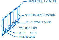
STAIR DETAIL
