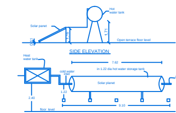
SIDE ELEVATION
