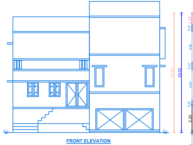
FRONT ELEVATION
