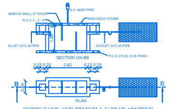
SECTION ON BB
