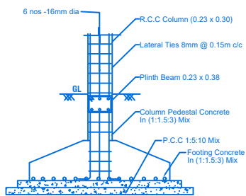
COLUMN FOOTING DETAILS
