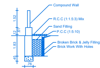
RAIN WATER HARVEST DETAILS
