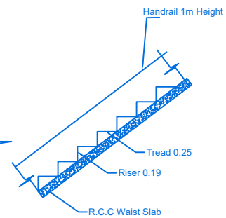
STAIR DETAILS
