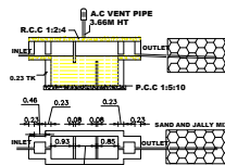
SEPTIC TANK AND TRENCH
