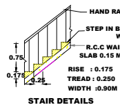
STAIR DETAILS
