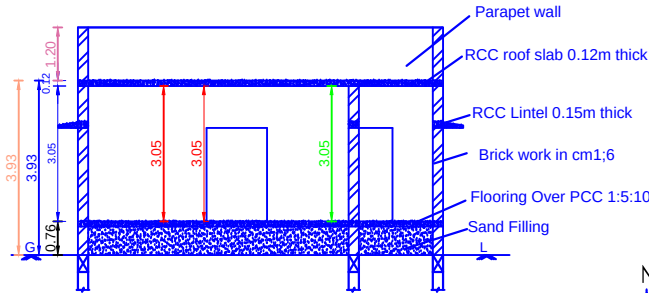
SECTION ON 'V-B'
