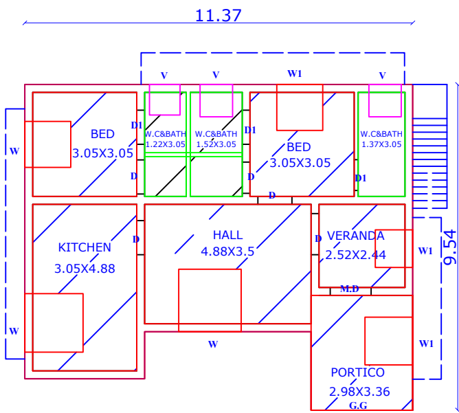
EXG-GROUND FLOOR PLAN DOOR NO:4/134B
