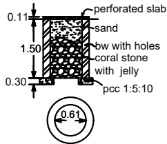
percolation pit
