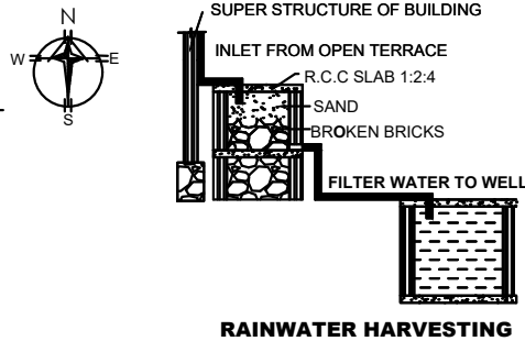
RAINWATER HARVESTING
