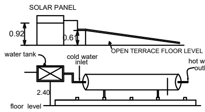
Details of solar water heating system
