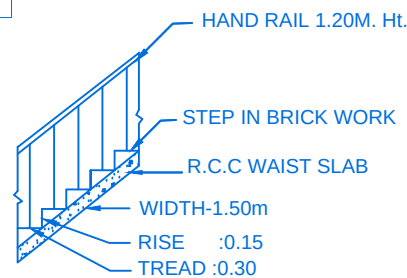
STAIR DETAIL
