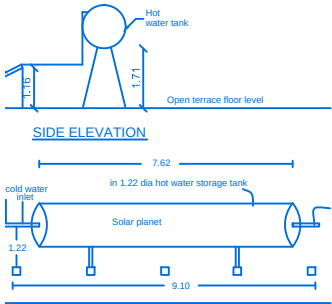
SOLAR WATER HEATER PLANT
