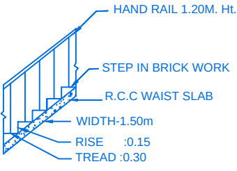
STAIR DETAIL
