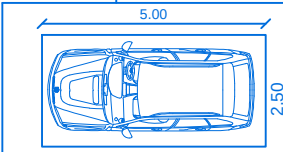
CAR POCKET DETAILS
