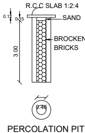
PERCOLATION PIT
