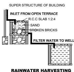
RAINWATER HARVESTING
