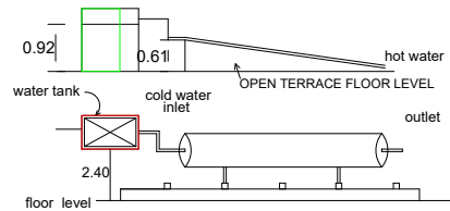
Details of solar water heating system
