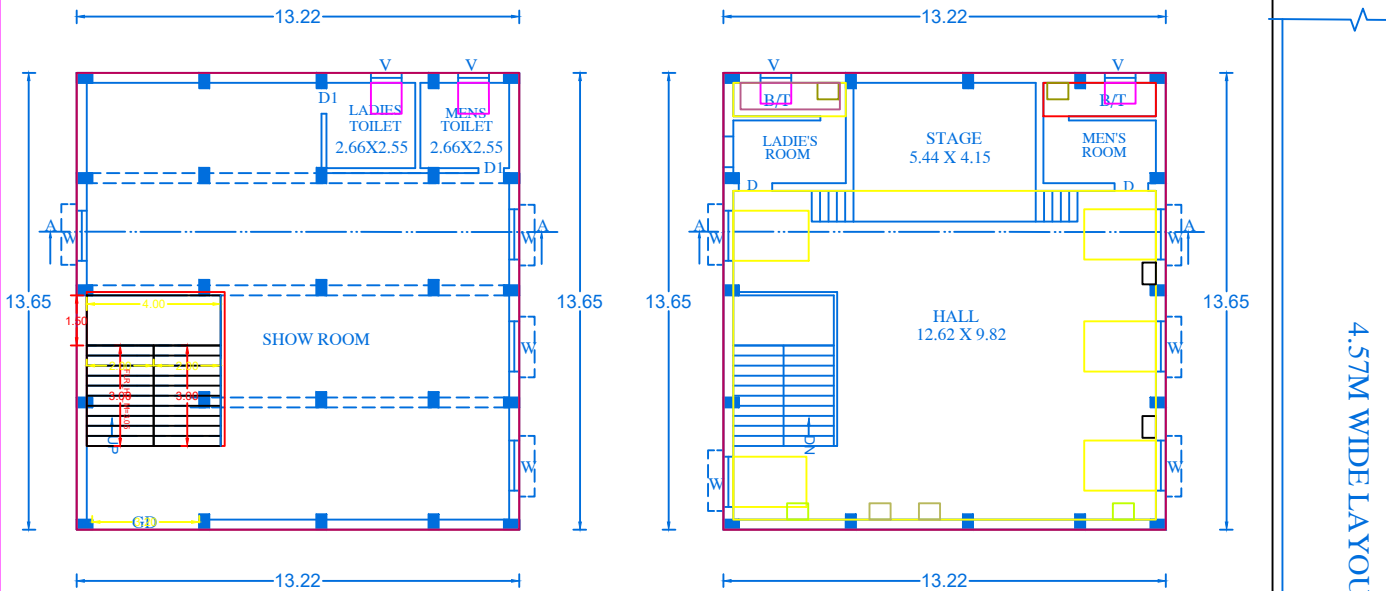
EX.GROUND FLOOR PLAN
