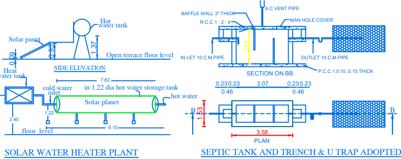
SOLAR WATER HEATER PLANT
