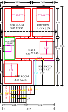
PLAN
