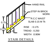
STAIR DETAILS
