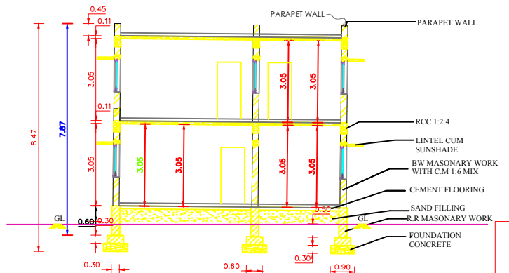
SECTION - A
