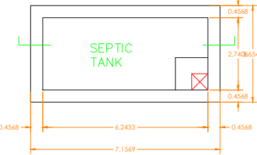
PLAN OF SEPTIC TANK SCALE 1"=2'-0"
