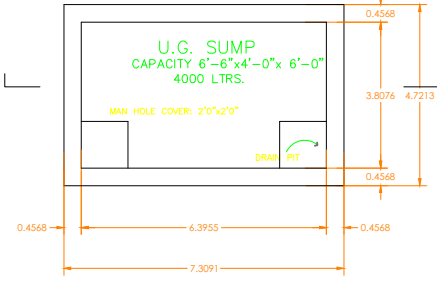
SUMP DETAIL SCALE 1"=4'-0"
