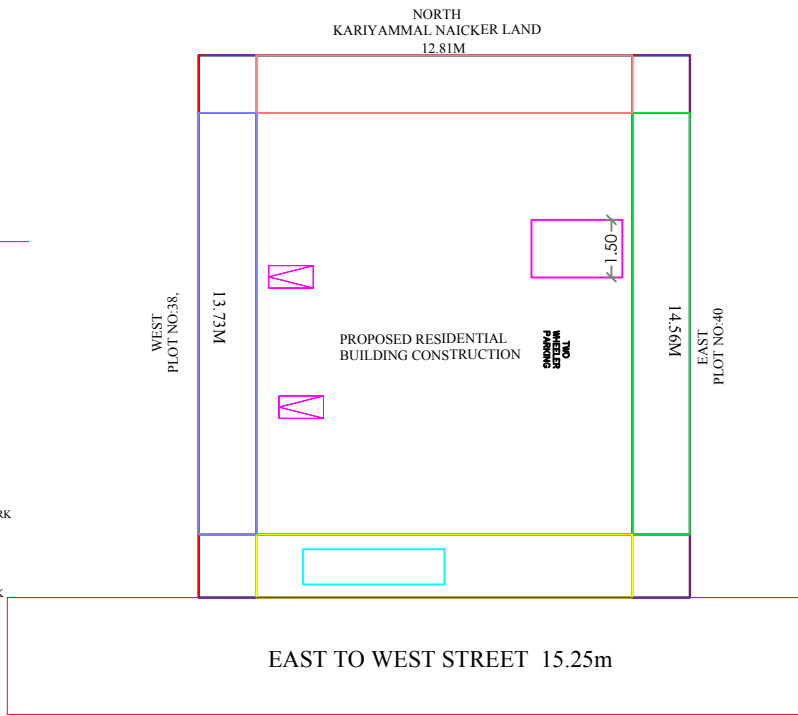
SITE PLAN
