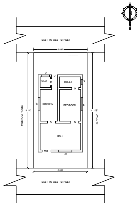
SITE PLAN
