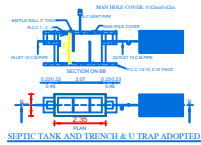
SEPTIC TANK AND TRENCH & U TRAP ADOPTED
