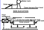
SOLAR WATER HEATER PLANT
