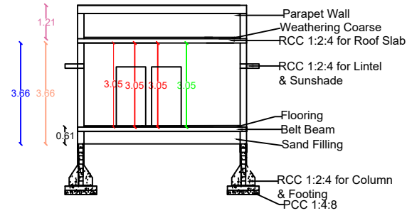
SECTION AB
