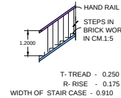
DETAILS OF STAIRCASE
