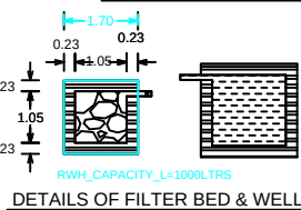
DETAILS OF FILTER BED & WELL
