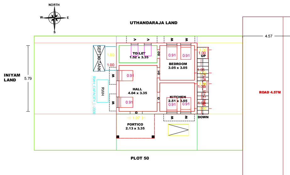
SITE PLAN FOR THE PROPOSAL
