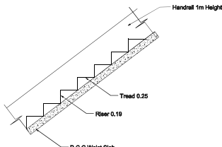
STAIR DETAILS
