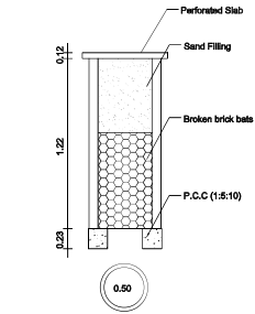
RAIN WATER COLLECTION WELL
