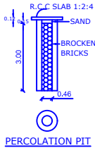
PERCOLATION PIT
