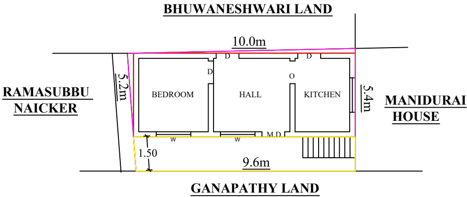
SITE PLAN(1:100)
