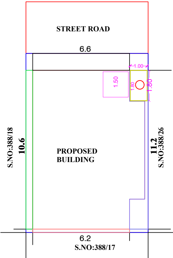
SITE PLAN
