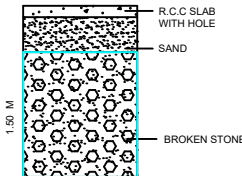
RAIN WATER HARVEST COLLECTION PIT.
