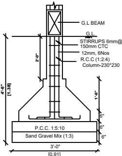
R.C.C. COLUMN FOOTING DETAILS
