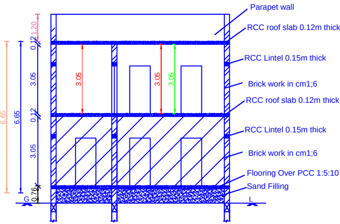
SECTION ON 'V-B'
