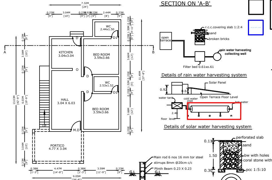
Details of solar water harvesting system
