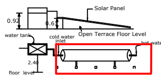
Details of solar water harvesting system
