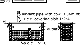
Details of septic tank & trench
