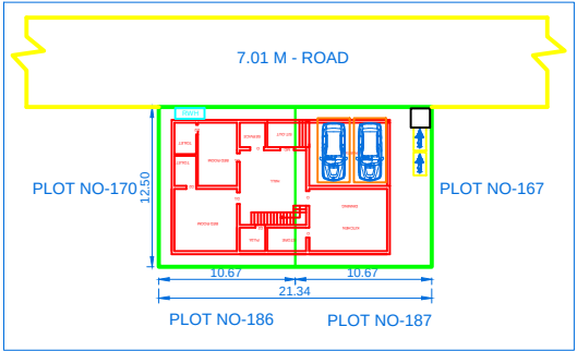
LOCATION PLAN Scale 1:400
