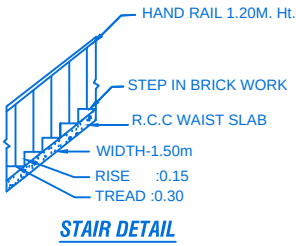
STAIR DETAIL
