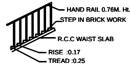
STAIR CASE DETAIL
