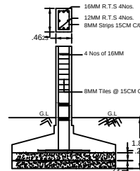
RCC COLUMN DETAILS
