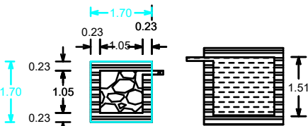
DETAILS OF FILTER BED & WELL
