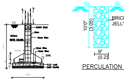
FOUNDATION DETAILS
