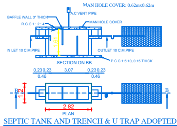
SECTION ON BB
