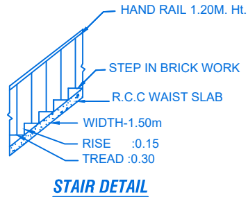
STAIR DETAIL
