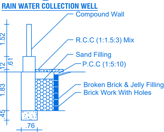
RAIN WATER HARVEST DETAILS
