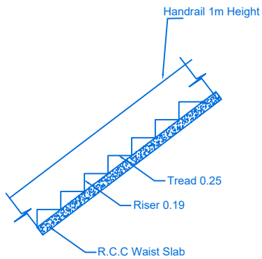
STAIR DETAILS
