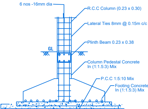
COLUMN FOOTING DETAILS
