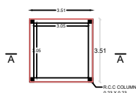
PLAN (WATER TANK-17)
