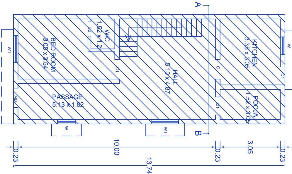
GROUND FLOOR
