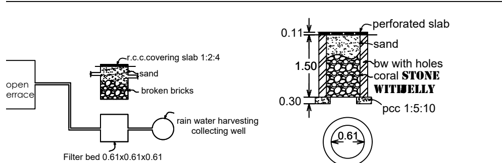
DETAILS OF RAIN WATER HARVESTING SYSTEM percolation pit
