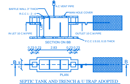
SEPTIC TANK AND TRENCH & U TRAP ADOPTED
