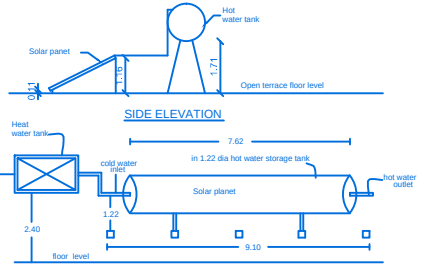
SOLAR WATER HEATER PLANT
