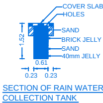
SECTION OF RAIN WATER COLLECTION TANK PLAN
