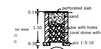
Percolation pit
