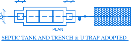
SEPTIC TANK AND TRENCH & U TRAP ADOPTED
