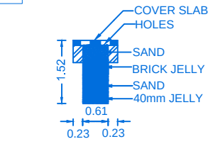
SECTION OF RAIN WATER COLLECTION TANK
