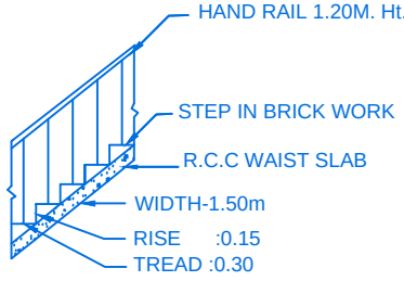
STAIR DETAIL
