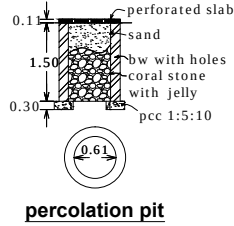
percolation pit
