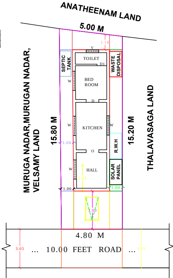
SITE PLAN (1:100)
