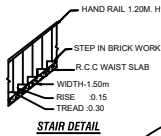
STAIR DETAIL
