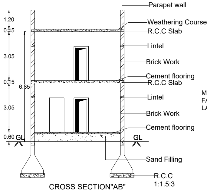
CROSS SECTION"AB"
