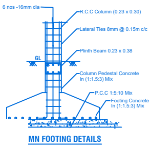
MN FOOTING DETAILS
