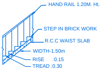
STAIR DETAIL
