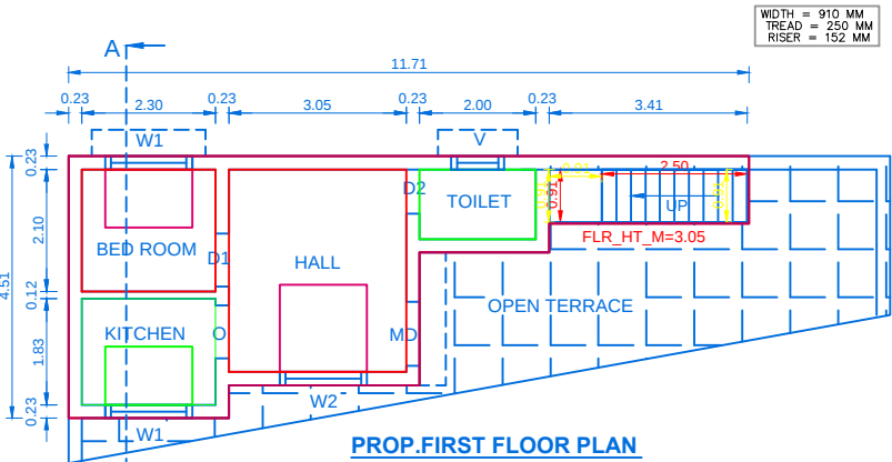
PROP.FIRST FLOOR PLAN
