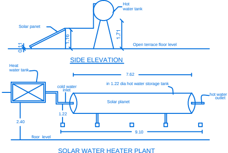
SOLAR WATER HEATER PLANT
