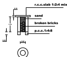
PERCOLATION PIT
