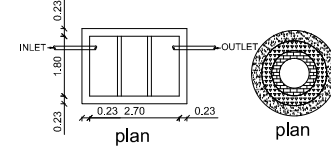
SEPTIC TANK DETAILS
