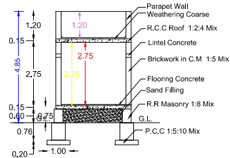
SECTION ON SS
