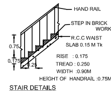
STAIR DETAILS
