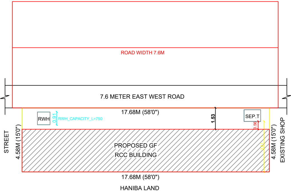
SITE PLAN
