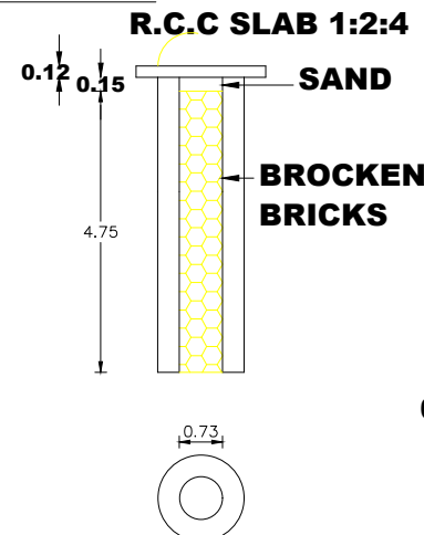
PERCOLATION PIT
