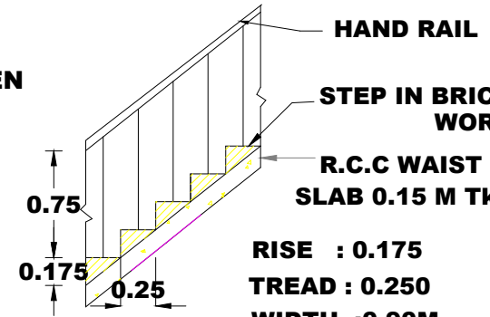
STAIR DETAILS
