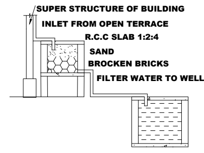
DETAILS OF FILTER BED & WELL
