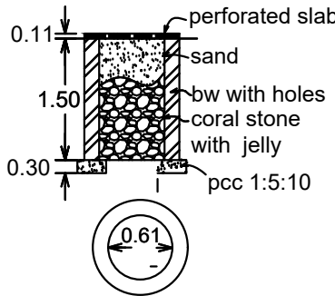
percolation pit
