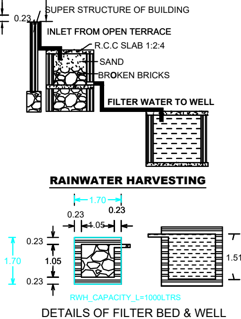
DETAILS OF FILTER BED & WELL
