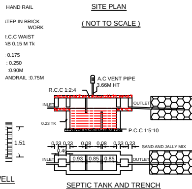
SEPTIC TANK AND TRENCH
